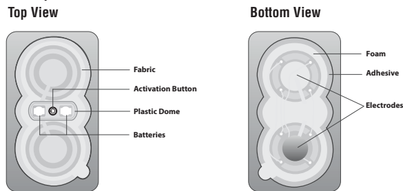
Figure 2: Iontophoretic Device
